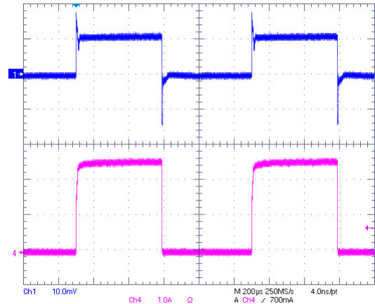
VIN=1.8V, VCNTL=3.3V, VOUT=0.9V @ 2.5A Sinking
