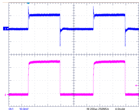
VIN=1.8V, VCNTL=5V, VOUT=0.9V @ 2.5A Sinking
