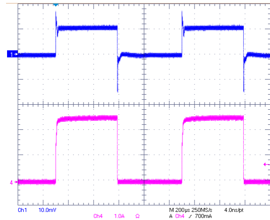
VIN=1.5V, VCNTL=3.3V, VOUT=0.75V @ 2.5A Sinking
