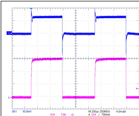
VIN=1.8V, VCNTL=3.9V @ 3A Sinking
