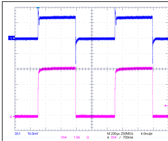
VIN=2.5V, VCNTL=5V, VOUT=1.25V @ 3A Sinking
