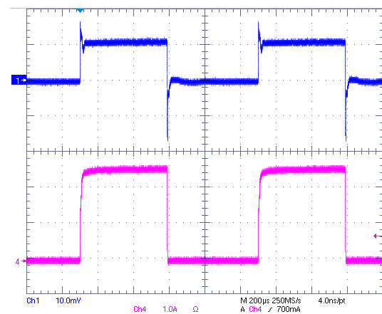
VIN=1.2V, VCNTL=3.3V, VOUT=0.6V @ 2.5A Sinking
