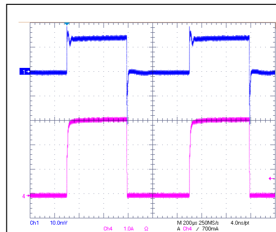
VIN=1.2V, VCNTL=3.3V, VOUT=0.6V @ 3A Sinking
