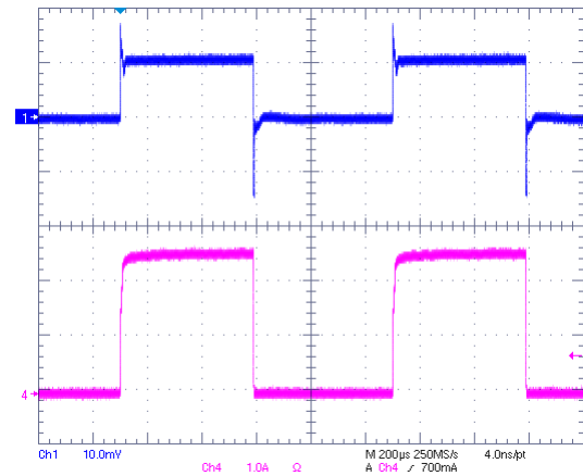
VIN=1.5V, VCNTL=5V, VOUT=0.75V @ 2.5A Sinking
