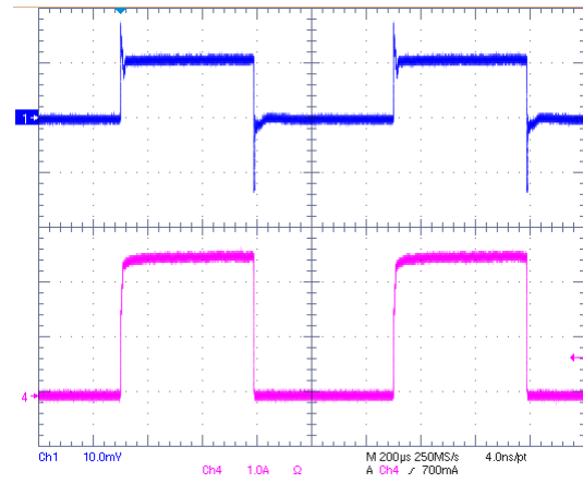
VIN=2.5V, VCNTL=5V, VOUT=1.25V @ 2.5A Sinking
